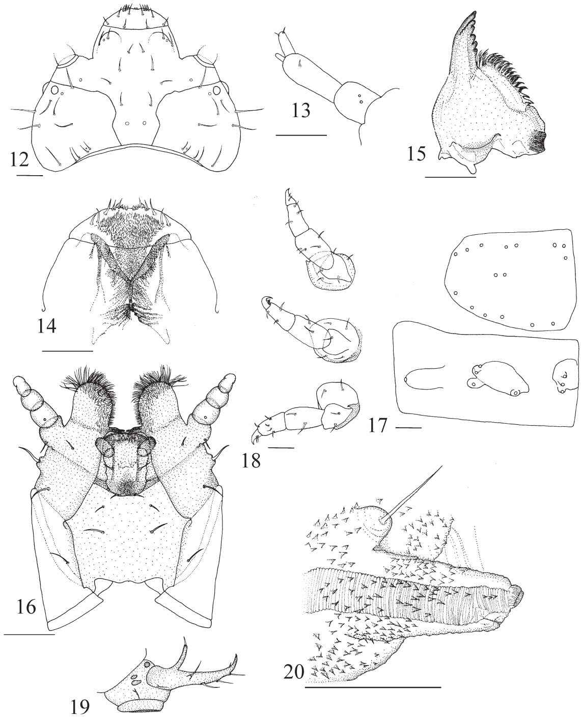
Figures 12-20. Soronia oculata , mature larva. Fig. 12 , head capsule, dorsal view; Fig. 13 , antenna; Fig. 14 , epipharynx, ventral view; Fig. 15 , mandible, dorsal view; Fig. 16 , maxillary-labial complex, ventral view; Fig. 17 , diagrammatic outline of pro-mesothoracic terga showing setal bases and outlines of tergal plates; Fig. 18 , legs, ventrolateral views; Fig. 19 , urogomphus, lateral view; Fig. 20 , spiracular tubercle and surface texture of A8.
