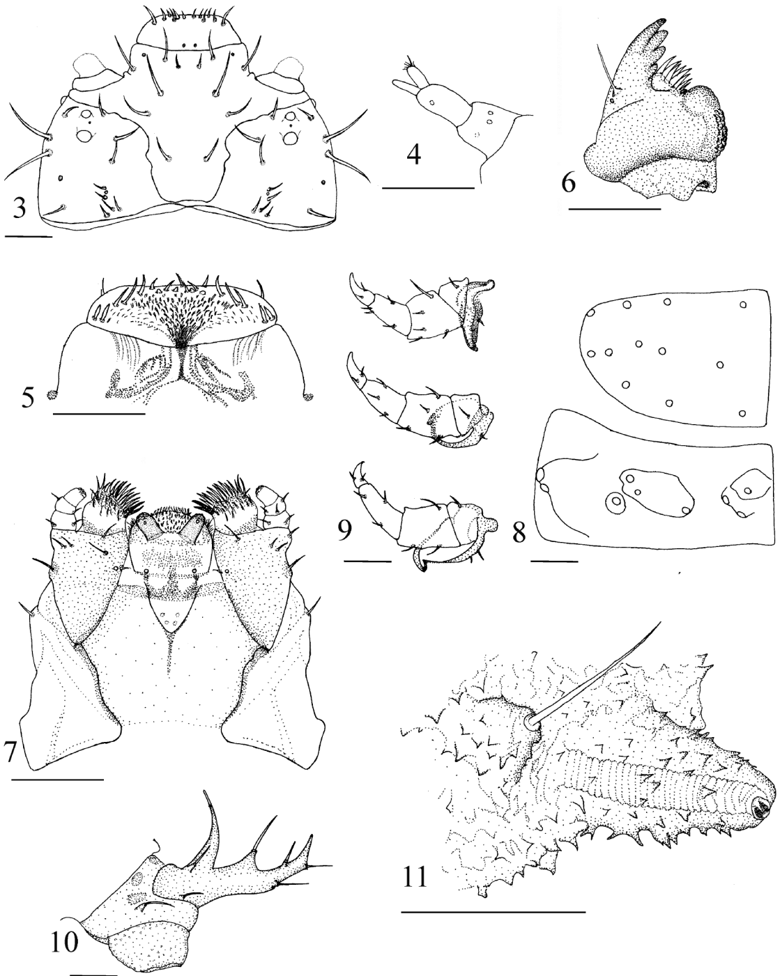
Figures 3-11. Hisparonia hystrix , mature larva. Fig. 3 , head capsule, dorsal view; Fig. 4 , antenna; Fig. 5 , epipharynx, ventral view; Fig. 6 , mandible, dorsal view; Fig. 7 , maxillary-labial complex, ventral view; Fig. 8 , diagrammatic outline of pro-mesothoracic terga showing setal bases and outlines of tergal plates; Fig. 9 , legs, ventral views; Fig. 10 , urogomphus, lateral view; Fig. 11 , spiracular tubercle and surface texture of A8.
